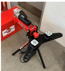
Bending device (for Ø10 and 16 mm)
